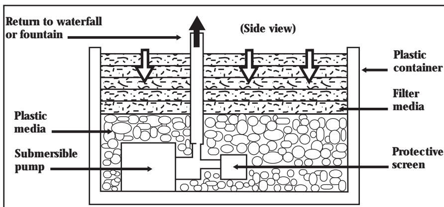
Figure 1. In-pond mechanical/bio-filter.
